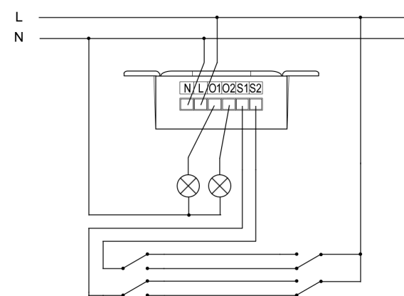
Circuit diagram, single gang switch, 2 circuits
