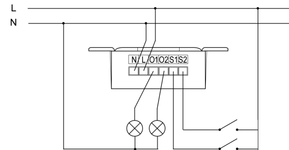
Circuit diagram, single gang switch, 2 circuits
